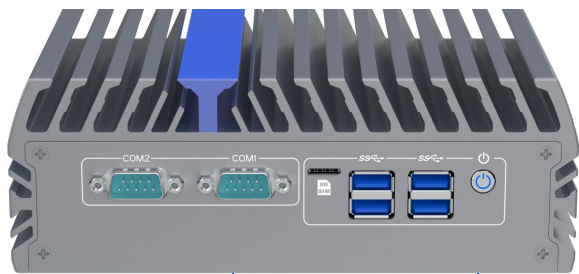
COM*2 SIM USB3.1x4 POWER
