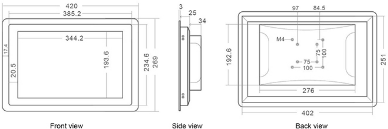
15.6" Touch Monitor
