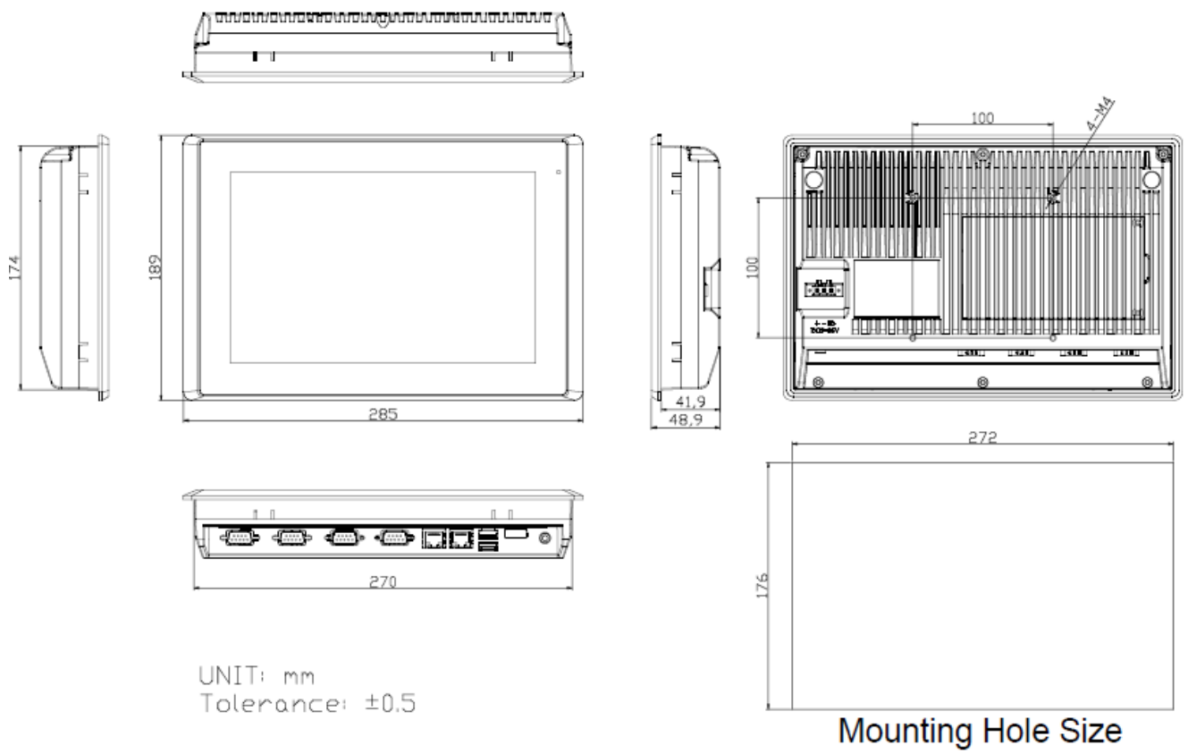
Figure 1.3: Dimensions of ARCHMI-710
