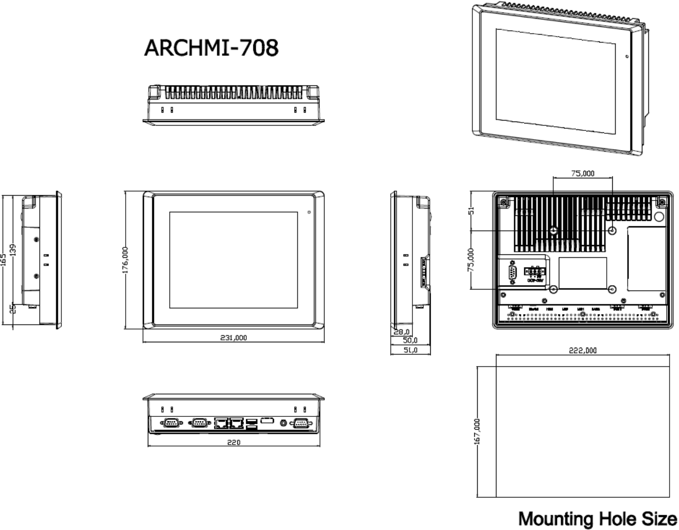
Figure 1.2: Dimensions of ARCHMI-708
