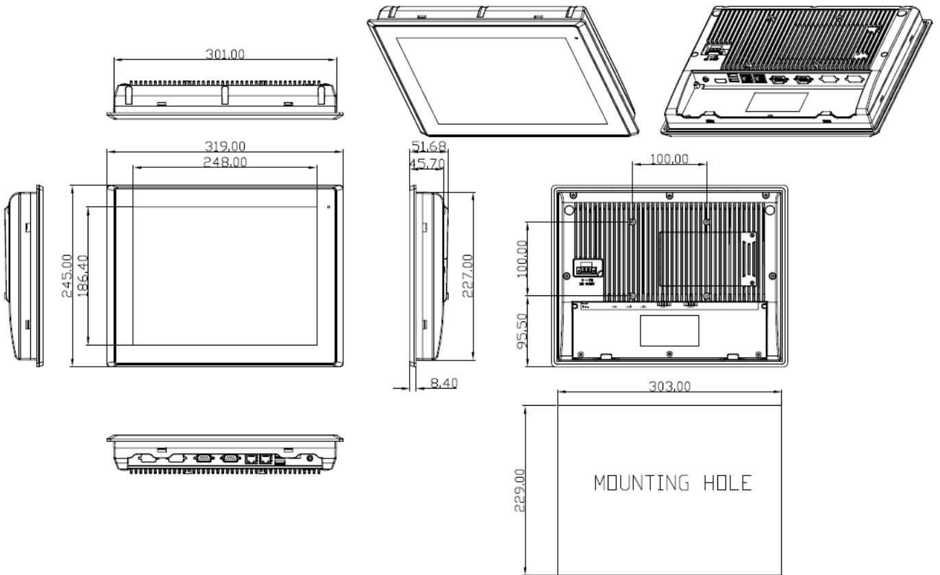
Figure 1.4: Dimensions of ARCHMI-712
