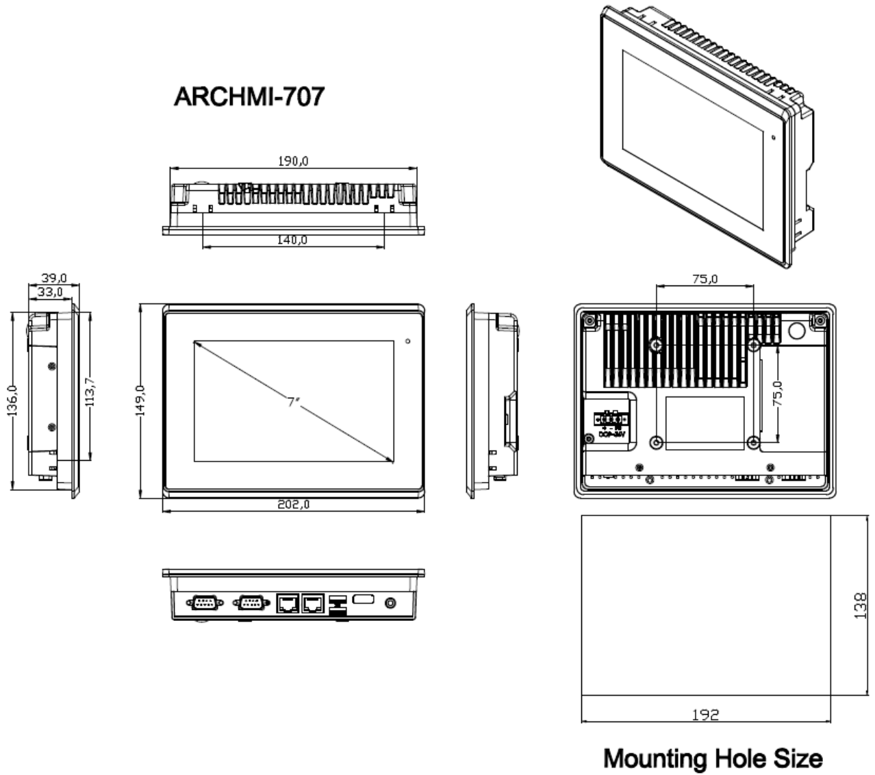
Figure 1.1: Dimensions of ARCHMI-707
