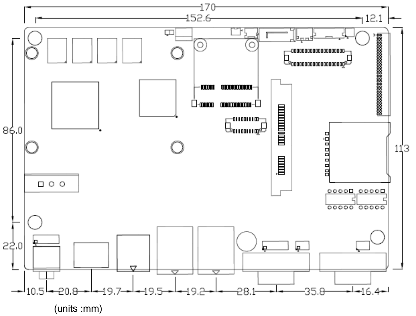
Figure 2.1: Mainboard Dimensions
