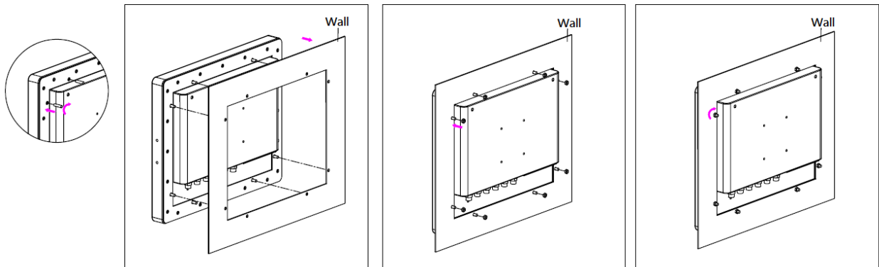
Figure 1.10: Panel Mounting of APC-3x94P/R
