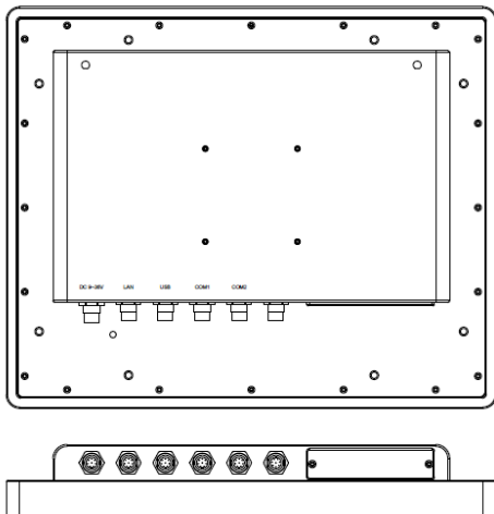
Figure 1.1: Dimensions of APC-3594P/R – Standard & Optional I/O APC-3X94P/R User Manual
